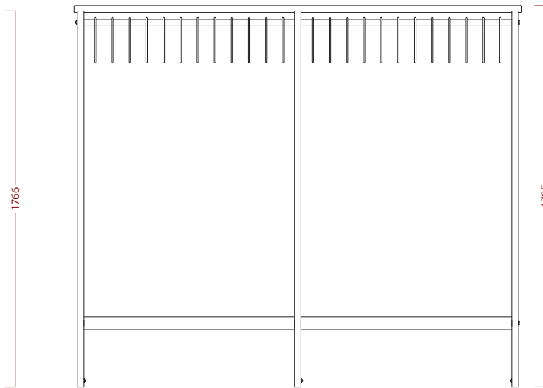
overall length as required equally spaced supports at maximum 1250mm centres
